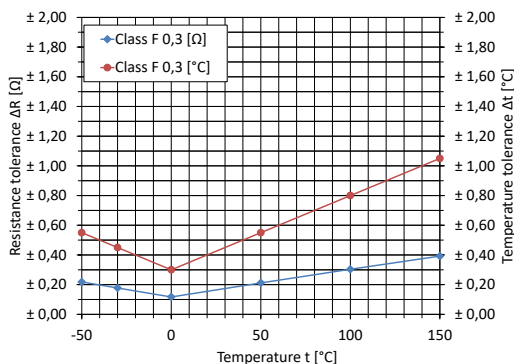
Picture 1: Resistance and temperature tolerances of Pt100
