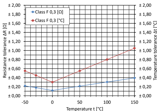
Picture 1: Resistance and temperature tolerances of Pt100
