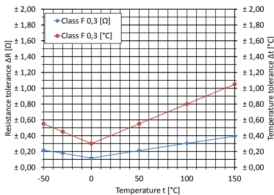
Picture 1: Resistance and temperature tolerances of Pt100
