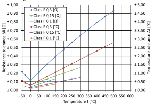
Picture 1: Resistance and temperature tolerances of Pt100 (Please note - the permitted operating temperature range depends on lead material!)
