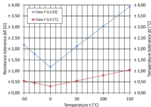
Picture 1: Resistance and temperature tolerances of Pt1000
