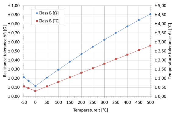
Picture 1: Resistance and temperature tolerances of Pt100 TC3750 ppm/K (Please note - the operating temperature range depends on lead material!)
