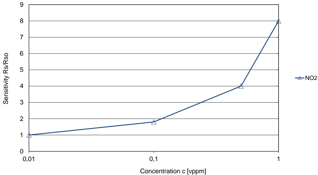
Figure 1: GGS 5430 T - Sensitivity characteristics on exposure to NO 2 (T H = 275 °C)
