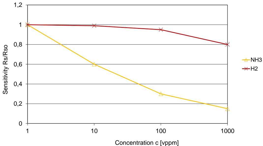
Figure 1: GGS 4430 T - Sensitivity characteristics on exposure to NH 3 and H 2 (T H = 470 °C)
