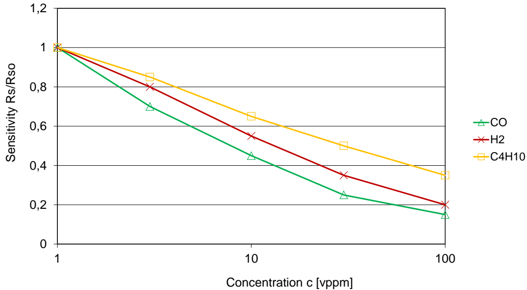
Figure 1: GGS 10530 T - Sensitivity characteristics on exposure to CO, H 2 and C 4 H 10 (T H = 350 °C)
