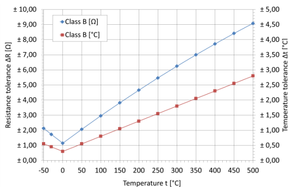
Picture 1: Resistance and temperature tolerances of Pt1000, TC 3750 ppm/K (Please note - the operating temperature range depends on lead material!)
