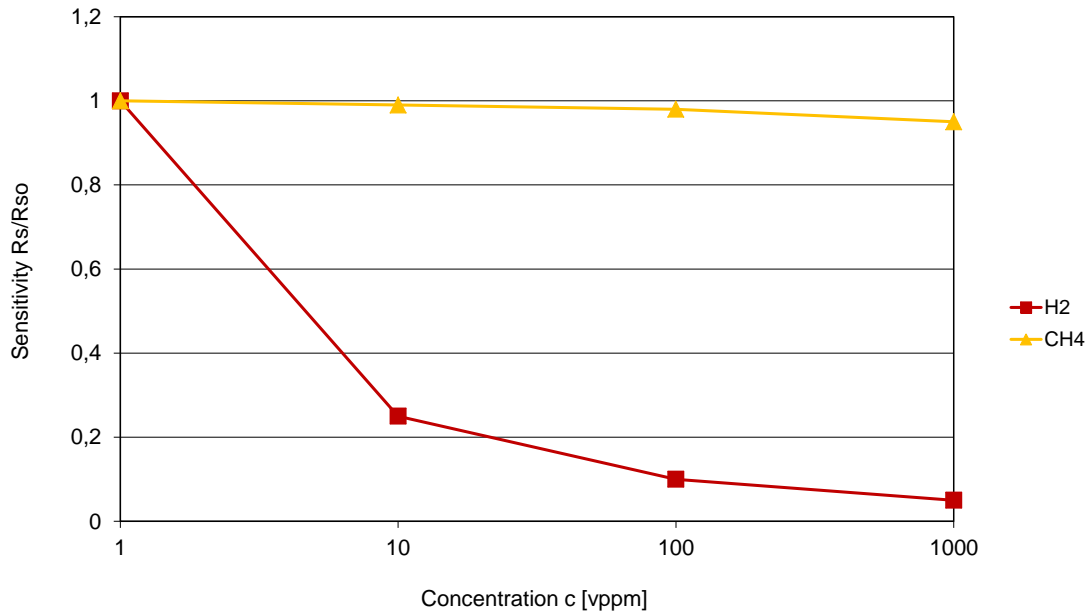
Figure 1: GGS 6530 T - Sensitivity characteristics on exposure to H 2 and CH 4 (T H = 475 °C)
